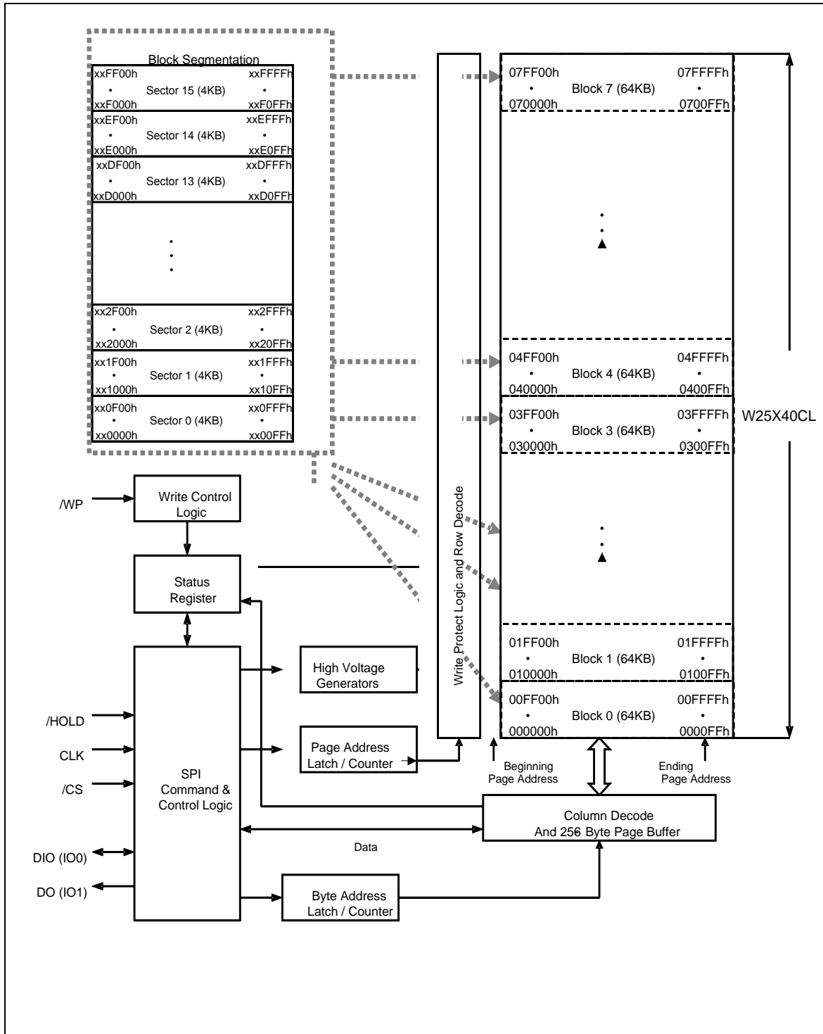
Figure 2. W25X40CL Serial Flash Memory Block Diagram
